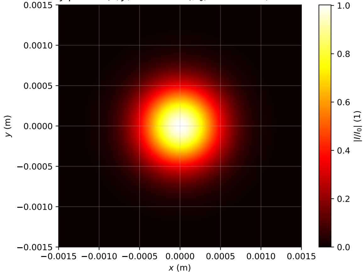
Intensity profile I(x, y, z = 0.398m)/I_0 , Pin=0.3Pcr, artificial time
